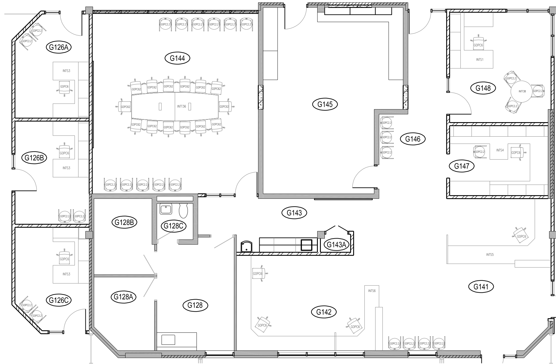
1 MAIN OFFICE FLOOR PLAN F1 1/8" = 1'-0"
